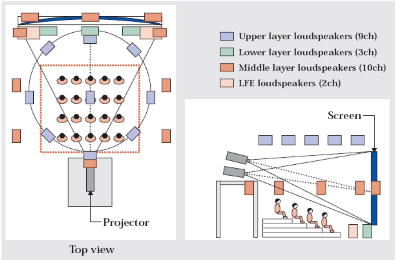
Figure 4: 22.2 channel audio system
