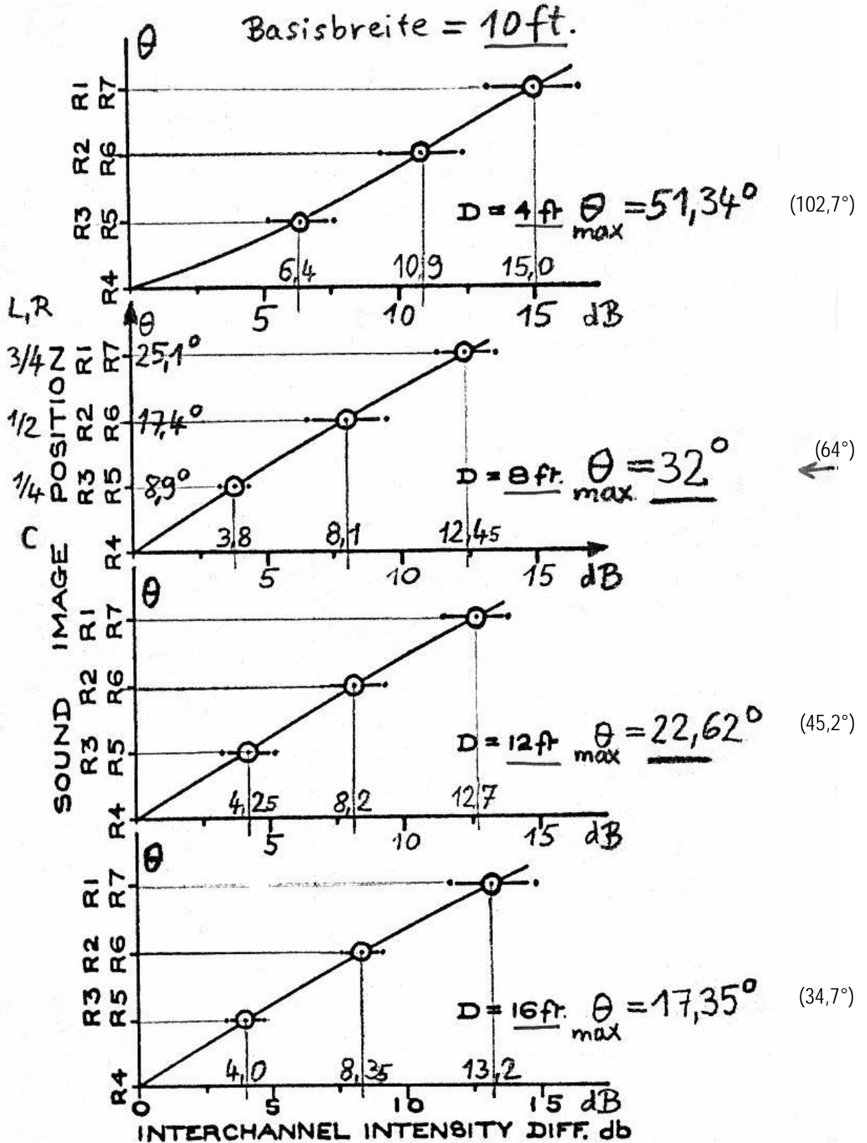
Fig. 5. Effect of variation of listening distance. \pm 51.3^\circ , \pm 32^\circ , \pm 22.6^\circ and 17.4^\circ . Central listening positions. 6 subjects tested. Half-curves only plotted.
